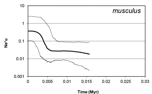
Fig. 8. Demographic history of M. m. domesticus , M. m. castaneus , and M. m. musculus population depicted as N_e \cdot \mu (effective population size*mutation rate) plotted against time (in million years) as estimated with the Bayesian skyline plot model. The thick middle line is the median estimate whereas the thin line indicates upper and lower limits of 95 % highest posterior density (HPD).
